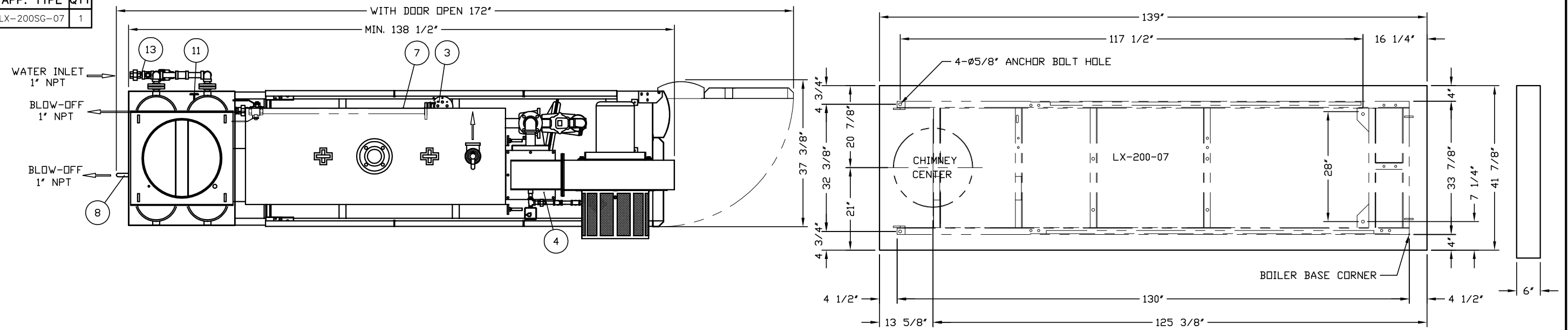
BOILER FOUNDATION
